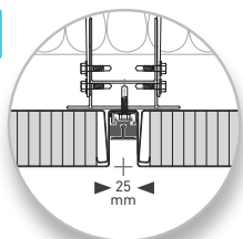
TRANSVERSAL JOINT
